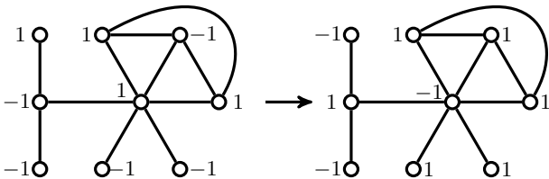
Figure 2: Left: the initial preferences of the nodes. Right: the resulting votes. For simplicity, the preference probabilities are not depicted.
