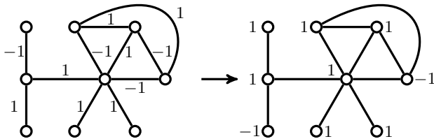
Figure 1: Left: the outcome of pairwise “conversations” between connected neighbors. Right: the resulting votes. For simplicity, the edge probabilities are not depicted.
